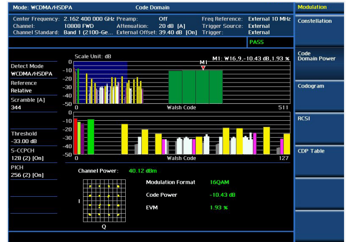
Modulation analysis — Code Domain Power
