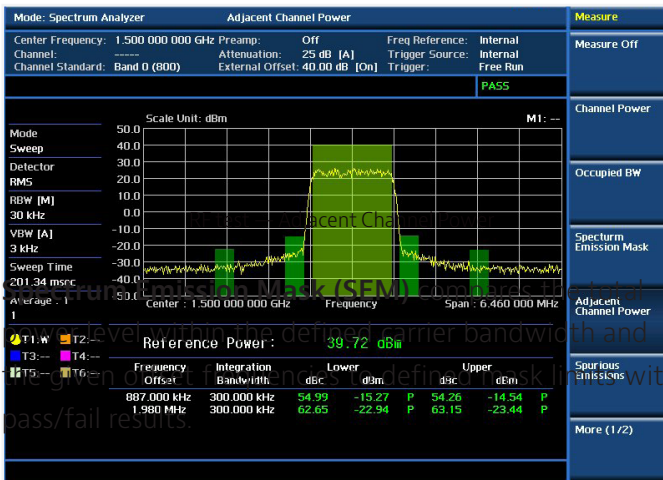
RF test — Spectrum Emission Mask
