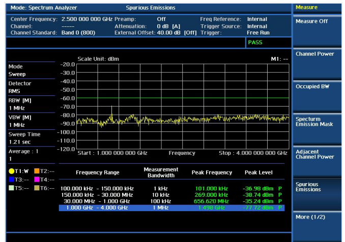
RF Test — Spurious Emissions
