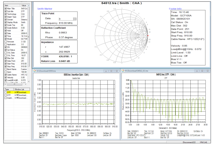
JDViewer VSWR, DTF, Smith chart
