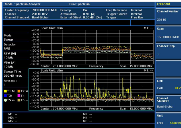
RF test — Dual Spectrum
