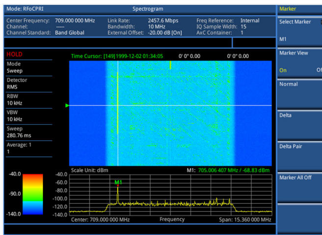
RfOCPRI – Spectrogram
