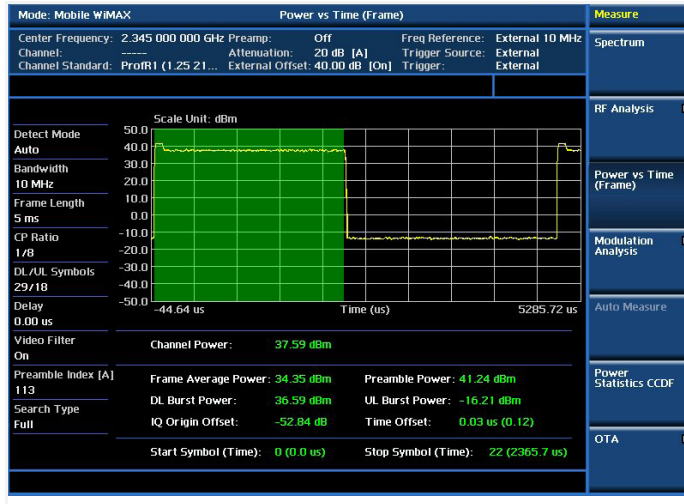
Modulation analysis — Power vs. Time
