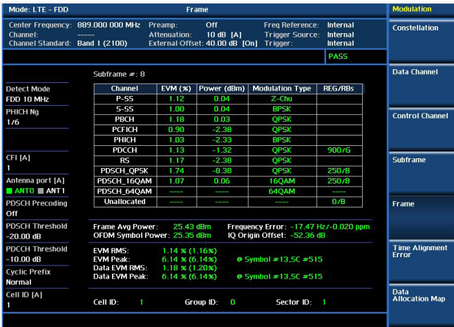
Modulation analysis — Frame
