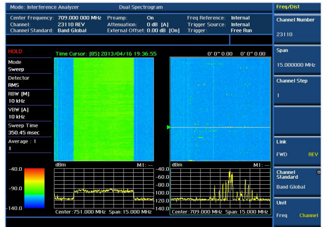
Interference analysis test — Dual Spectrogram
