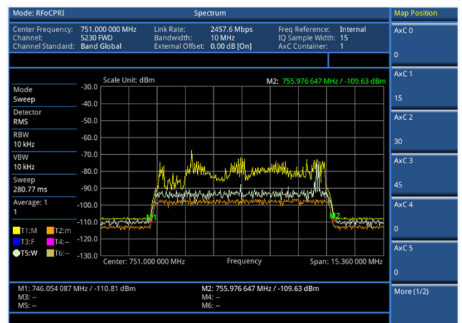
RfOCPRI – Spectrum
