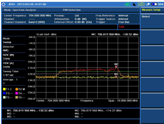
RF test — PIM Detection
