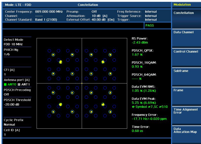
Modulation analysis — Data Constellation
