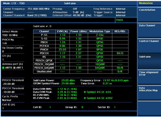
Modulation analysis — Subframe
