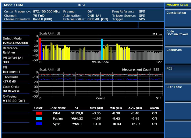
Modulation analysis — RCSI
