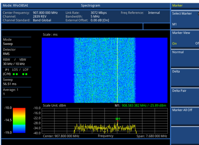
RfOBSAI – Spectrogram
